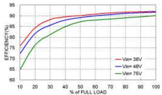
FED40-48S05 Efficiency VS Output Load
