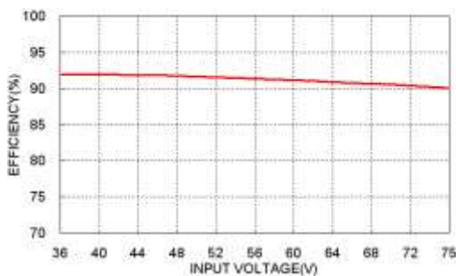
FED40-48S05 Efficiency VS Input Voltage
