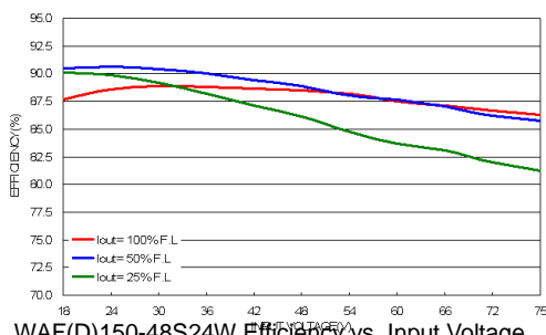
WAF(D)150-48S24W Efficiency vs. Input Voltage
