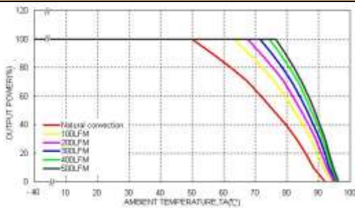
WAF(D)150-48S24W Derating Curve (Note 1)
