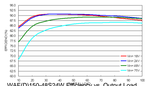
WAF(D)150-48S24W Efficiency vs. Output Load
